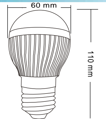
GN-HP-2835WW5W-G60-E27-SA
